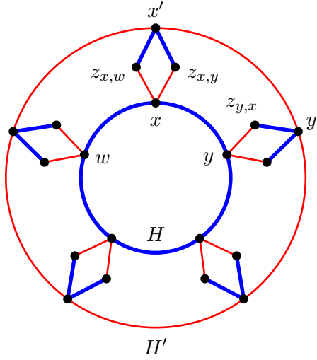
FIGURE 1. Sketch of a (C_5, C_5)_F -transformer built from five C_6 -switchers and five K_{2,2} -switchers.
