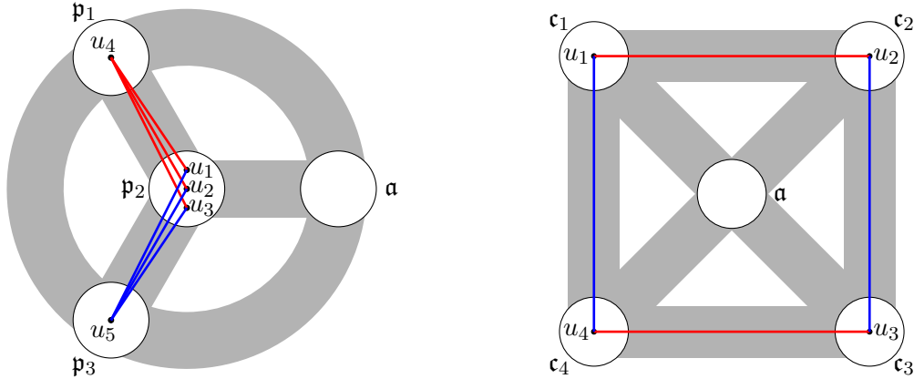
FIGURE 2. A 3-compressible (K_{2,3})_F -switcher with augmentation \{p_1, p_3\} and a 4-compressible (C_4)_F -switcher with augmentation \emptyset . The shaded areas indicate where the edges of the switchers may lie.
